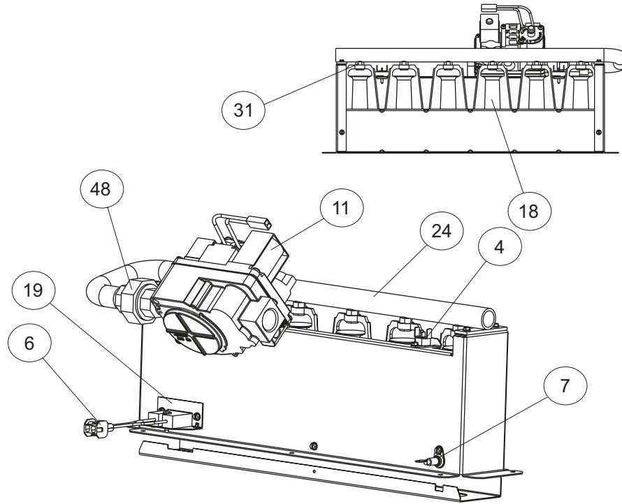
Figure 3: GAS CONTROLS
